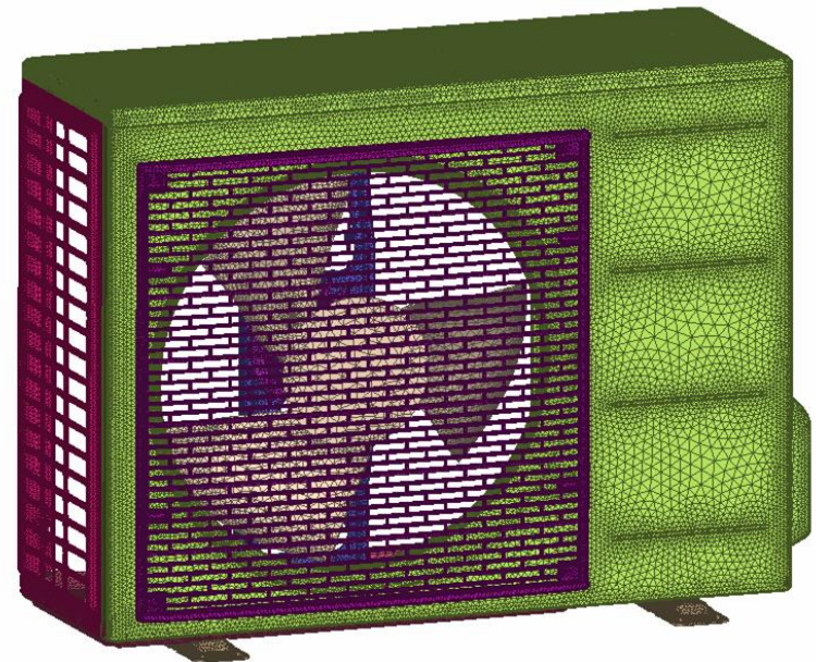
Detail of mesh on the grill
