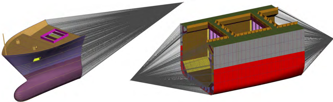
Fig.13: “Rigidized” models
