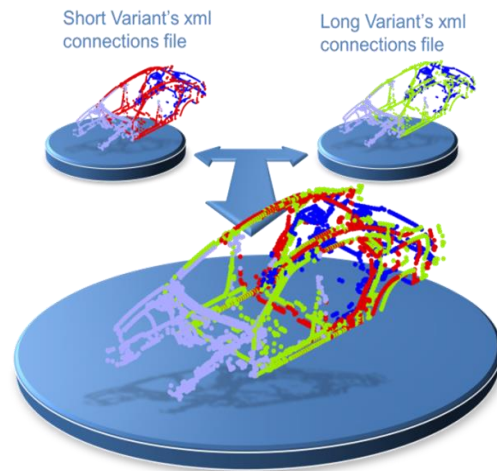
ANSA 150% Model Connection File
