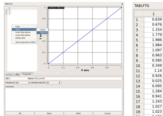
Definition of loads
