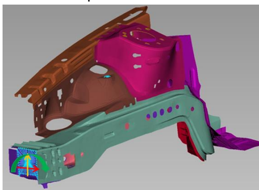
The shock tower of a vehicle body is subjected to two forces and a moment.
