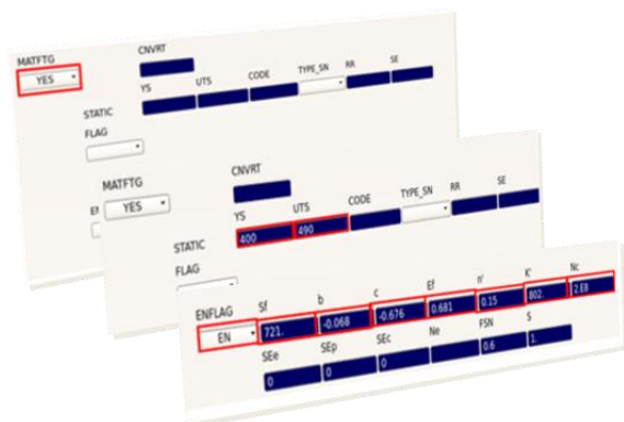
Defining the material properties in ANSA
