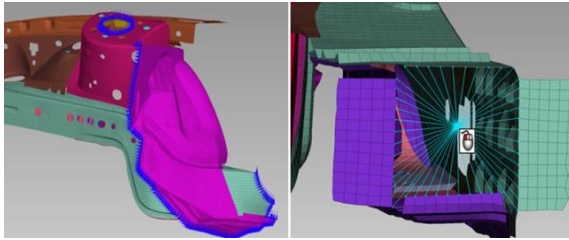
Definition of boundary conditions
