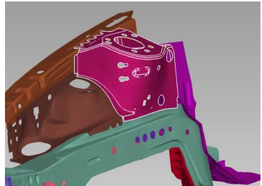
Definition of fatigue properties
