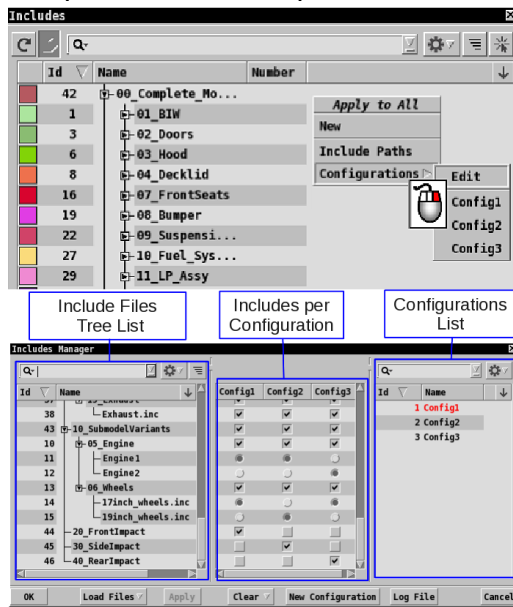
Figure 1: Include configurations creations and handling
